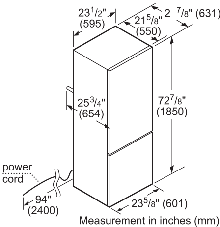
24" B10CB81NVW/B Dimensions
