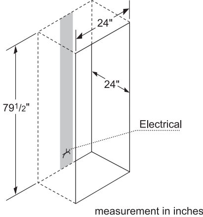
24" B11CB50SSS Installation
