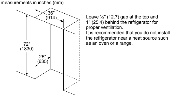
B36CL81ENG Installation
