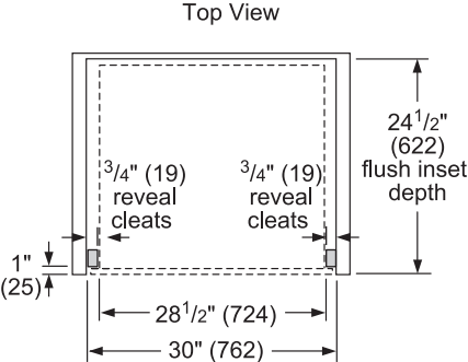
30" Flush Installation
