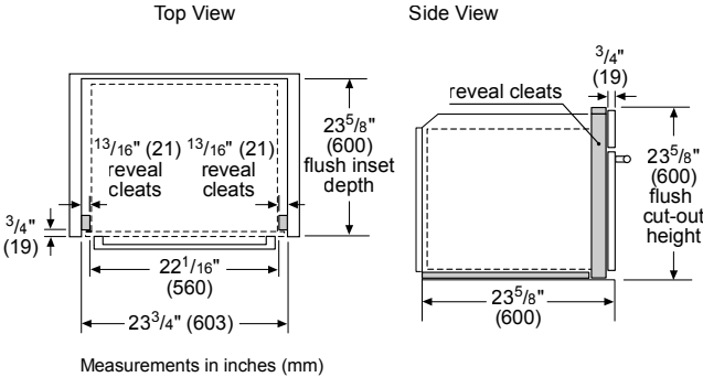
HBE5452UC Single Wall Oven Flush Installation
