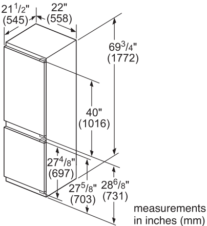
B09IB91NSP Dimensions
