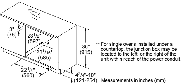
HBE5452UC Single Oven Under-Counter Installation
