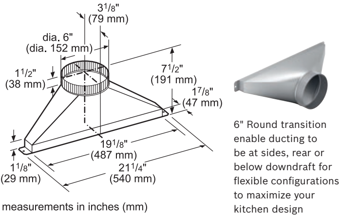
HDDSTRAN6 6" Side / Rear / Downward Transition for Downdraft
