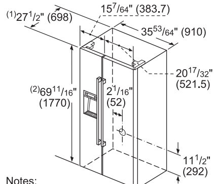
B20CS30SNS Dimensions
