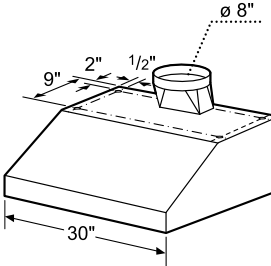
800 Series 30" DPH30652UC Under-Cabinet Hood
