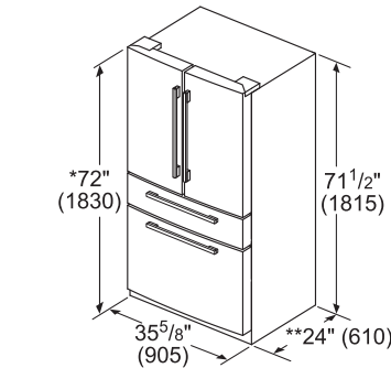
B36CL80SNS Dimensions
