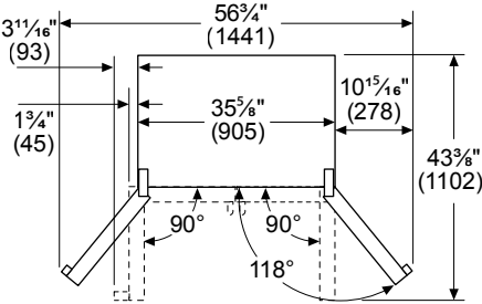
B36CL80SNS (Overhead Views)
