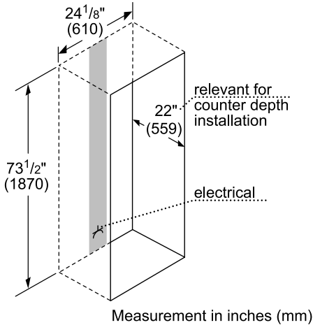
24" B10CB81NVW/B Installation
