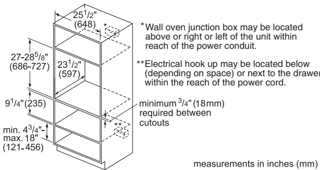
Standard Installation 27" Speed Oven or Microwave over Single Oven
