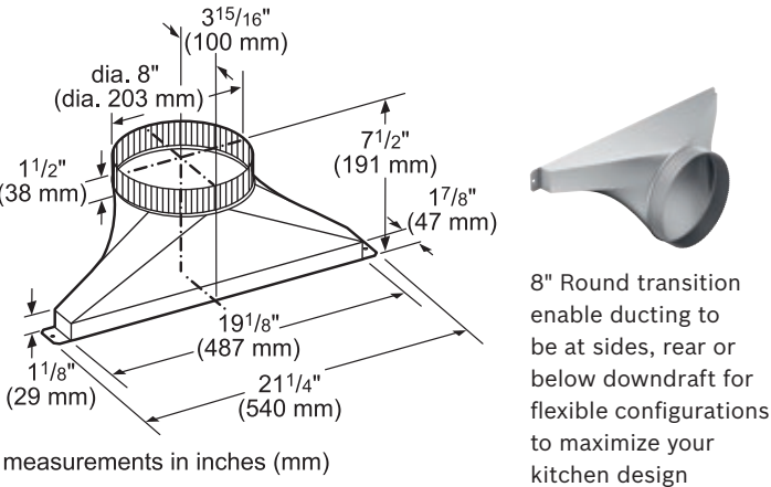
HDDSTRAN8 8" Side / Rear / Downward Transition for Downdraft
